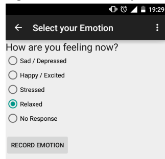
Figure 3: Self-report UI
