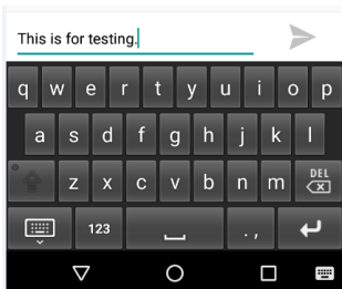
Figure 2: EmoReflect keyboard
